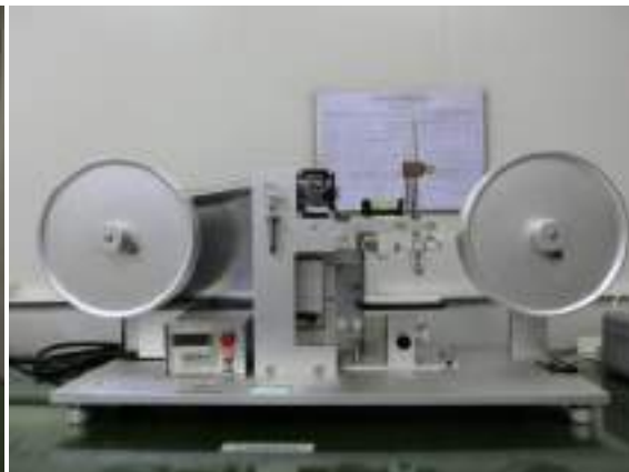
RCA耐磨測試儀 Paper tape abrasion tester
